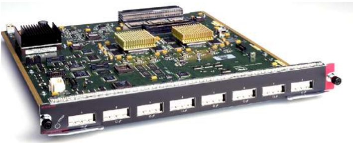
Figure 8. Classic Gigabit Ethernet Optical Interface Module WS-X6408A-GBIC
